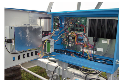
Inside the competitor's GPS control box/panel
