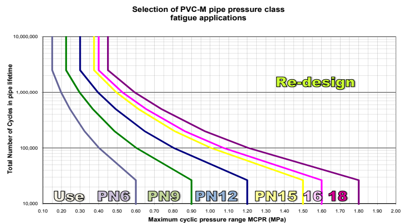
FIGURE 2 – Fatigue Design Chart for PVC-M Pipes
